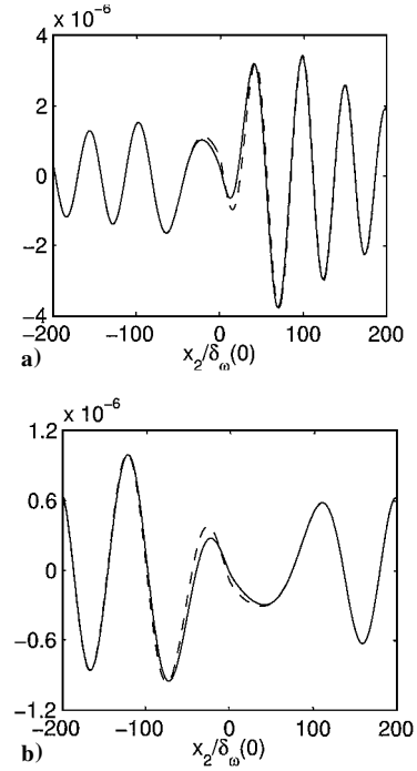
Fig. C3 Monopolar source in a sheared mean flow; transverse pressure profiles obtained using —, simplified LEE and ---, full LEE: a) x_1 = 0 and b) x_1 = 300\delta_\omega(0) .
