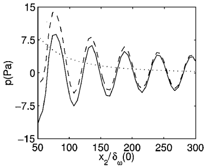
Fig. 14 Noise generated by a mixing layer; transverse pressure profiles obtained at x_1 = 90\delta_w(0) by solving LEE with source terms: —, S_1 - \overline{S_1} , ---, S_1 , and \cdots , S_2 .
