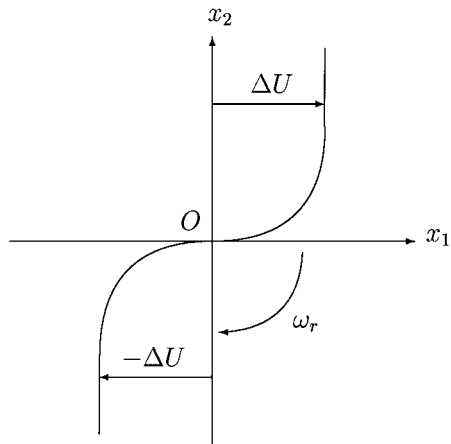
Fig. 7 Sheared mean flow with a zero convection velocity; two flow velocities \pm \Delta U and rotation of two corotating vortices shown by \omega_r .
