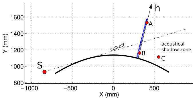
Figure 4: Plan view of the experiment, with the positions of the curved boundary, source and receivers.
