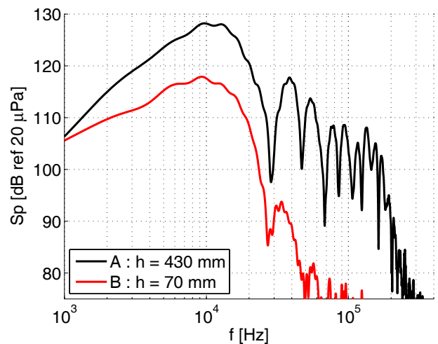
Figure 6: Spectra calculated from the measured waveforms (see figure 5), measured without turbulence. Black line : h = 43 cm (point A). Red line : h = 7 cm (point B).
