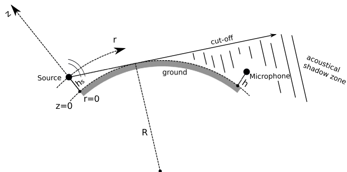
Figure 2: Formation of a shadow zone over a convex boundary.
