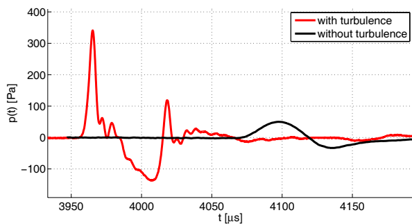
Figure 9: Example of measured waveform in point C, with a pressure level amplified by a factor 7. Red line : example of waveform in turbulent medium. Black line : reference waveform, measured at the same position without turbulence.
