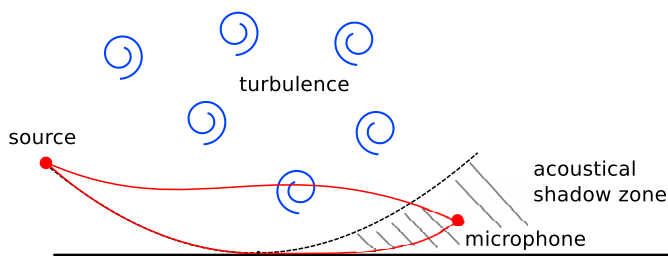
Figure 1: Two possible mechanisms of propagation into the shadow zone: diffraction on the ground, and scattering by turbulence.
