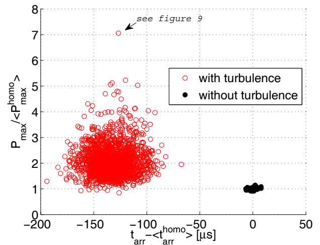
Figure 8: Scatter plot of P_{max} amplification factor P_{max} / \langle P_{max}^{homo} \rangle as a function of relative arrival time t_{arr} - \langle t_{arr}^{homo} \rangle , for every 2000 waveforms measured in point C with turbulence (red circles) in the shadow zone. \langle P_{max}^{homo} \rangle is the mean positive peak pressure without turbulence, and \langle t_{arr}^{homo} \rangle is the mean arrival time of the waves without turbulence, at the same position.
