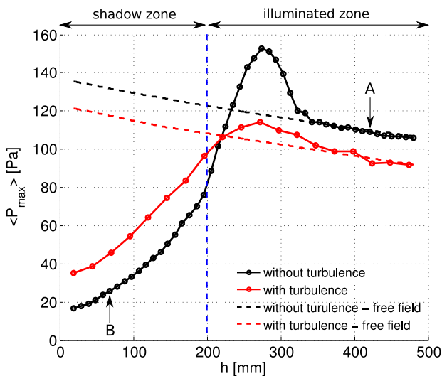
Figure 7: Measured positive peak pressure \langle P_{max} \rangle as a function of height h . Black solid line : homogeneous medium with the curved boundary. Black dashed line : homogeneous medium in free field. Red solid line : turbulent medium with the curved boundary. Red dashed line : turbulent medium in free field. The blue vertical dash line represents the geometrical limit of the shadow zone.
