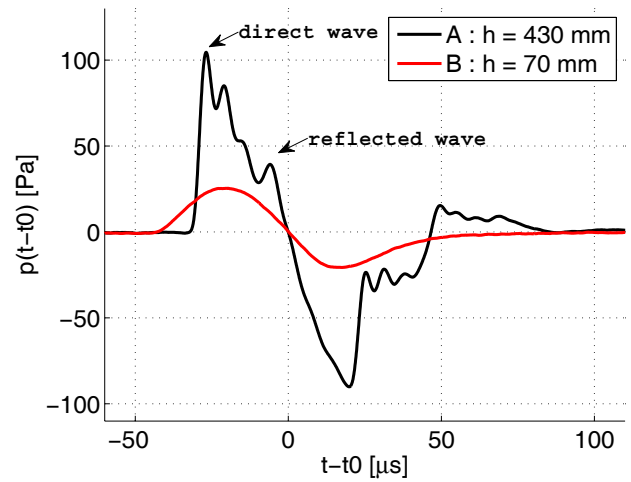
Figure 5: Examples of waveforms measured without turbulence. Black line : h = 43 cm (point A). Red line : h = 7 cm (point B).
