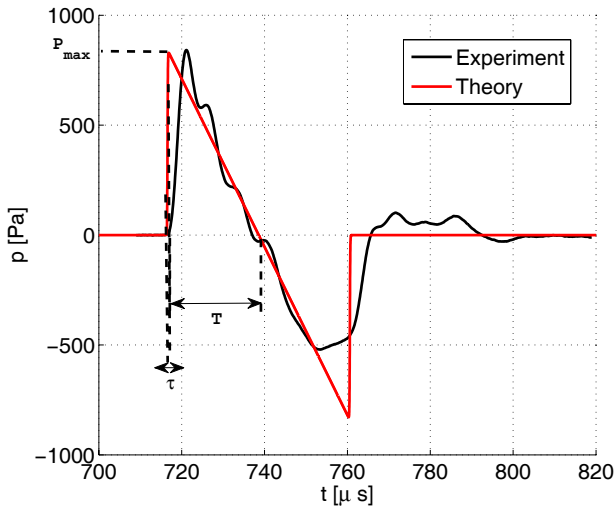
Figure 3: Theoretical waveform (red lines) at 30 cm from the spark source, and measured waveform at the same distance (black line). The positive peak pressure P_{max} , half-duration T and rise time \tau are defined.
