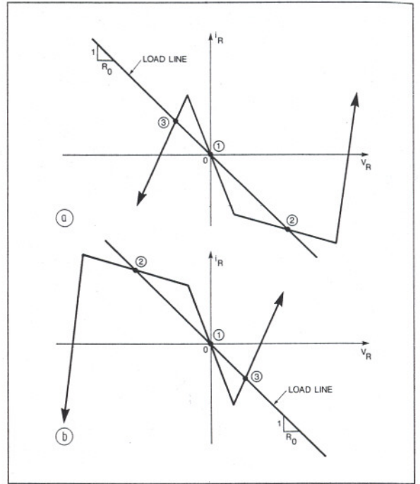
Fig. 8. The 2 dual 4-segment characteristic in (a) and (b) are the simplest eventually passive, hence physically realizable v_R - i_R characteristic which include that of Figs. 6(b) and 7(b) respectively, as a subset.
