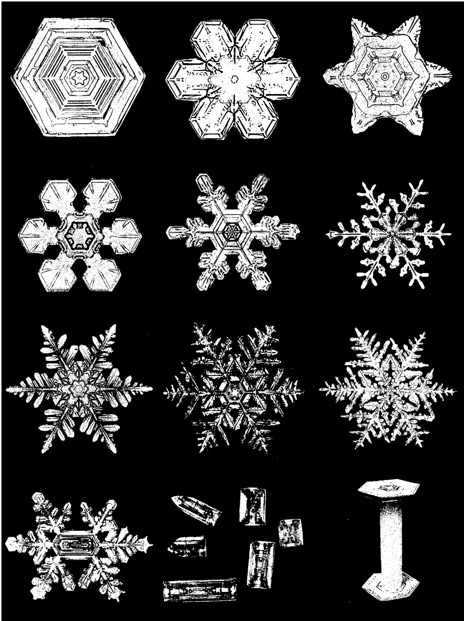
Fig. 1. Snow crystals: plates, sectors, stellar, dendrite, irregular and three dimensional.
