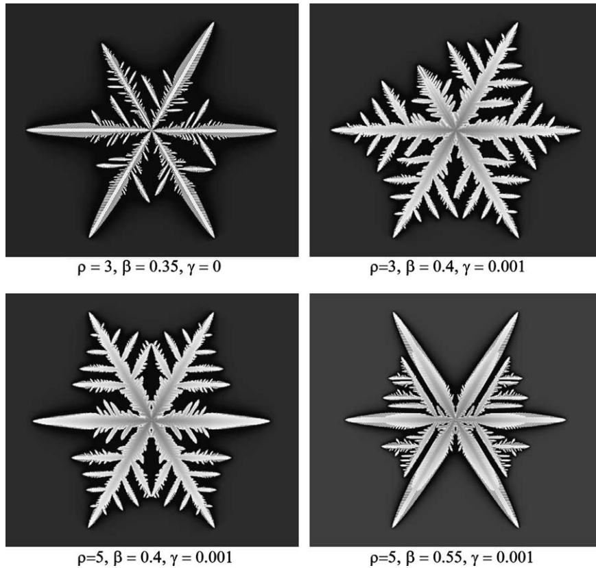
Fig. 6. Growth from a random initial cluster.
