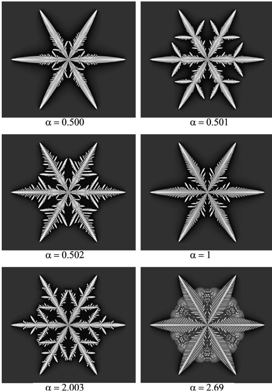
Fig. 5. Variety of forms appearing for different diffusion constants when \beta = 0.4 , \gamma = 0.0001 .
