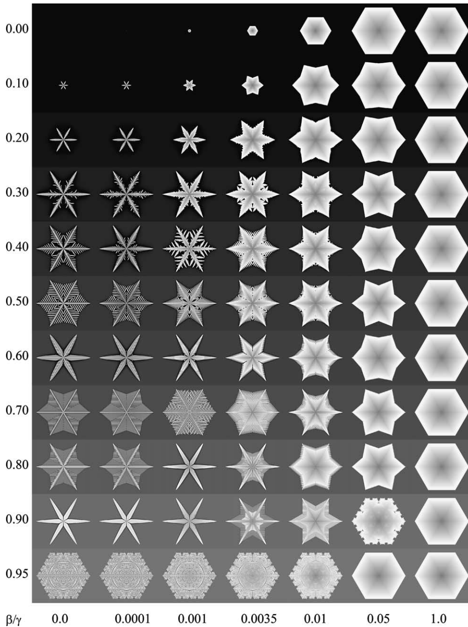
Fig. 3. Growth forms that appear as \beta and \gamma vary.
