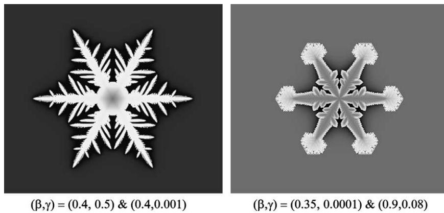
Fig. 7. Growth when parameters are changed.
