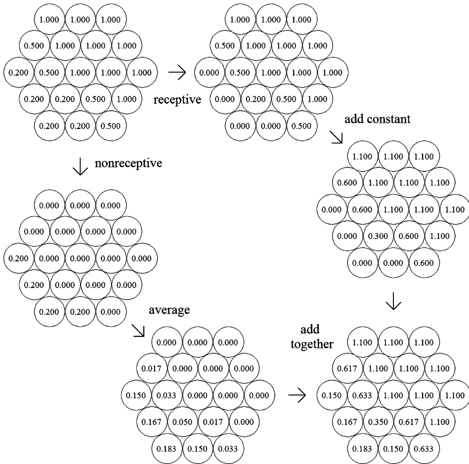
Fig. 2. Illustration of the algorithm on a small patch.
