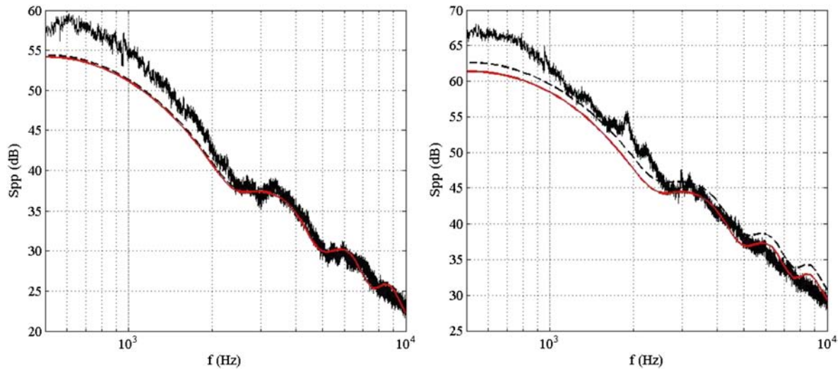
Fig. 5—Acoustic spectra of the optimized airfoil at z = 10/3d (left) and z = 4/3d (right). Measurements (thin) geometrical near-field expression (7) (red) and far-field expression (5) (dashed) for U = 15 m/s, TI = 0.05 , \Lambda = 0.009 m.
