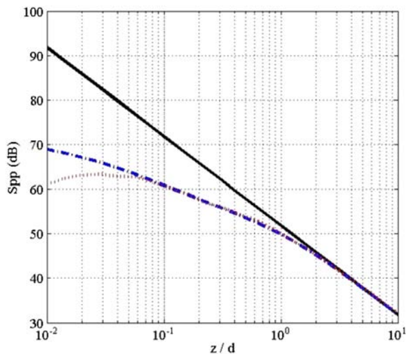
Fig. 3—Comparison of acoustic spectra at various distances, using Amiet's model (5) (solid), direct integration (3) (dots) and geometrical near-field correction (7) (dash-dots) for U = 30 m/s, TI = 0.05 , \Lambda = 0.009 m.
