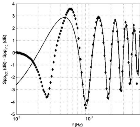
Fig. 7—Difference between the total and free-field spectra for the benchmark axial fan. Image method (solid) and ATV model (symbols). Observer is located at 0.2 m away on the rotation axis; plate is located parallel to the rotation plane, at 0.2 m away from the rotation center.
