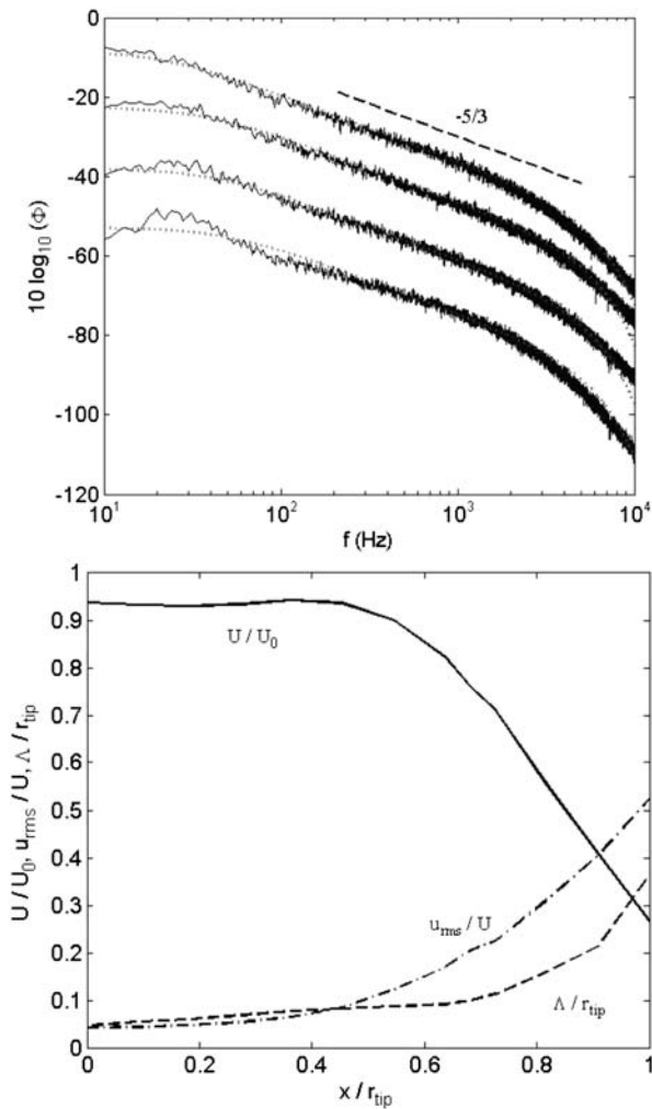
Fig. 9—Turbulence spectra at the strip centers on the rotation plane (top) measured (solid) and fitted von Karman model (dots) and corresponding flow profile (bottom) normalized velocity (solid), turbulent intensity (dash-dots) and modeled turbulent length scale 19 .
