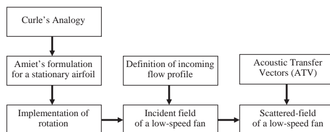
Fig. 1—Flowchart of the fan noise simulation.
