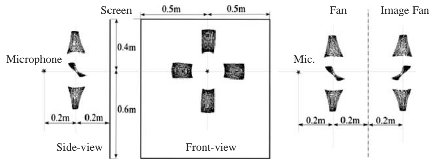
Fig. 6—Sketches of the scattering problem, ATV model (left) and Image Method (right).
