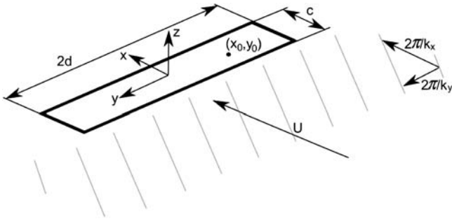
Fig. 2—A sketch of an airfoil swept by a skewed gust.
