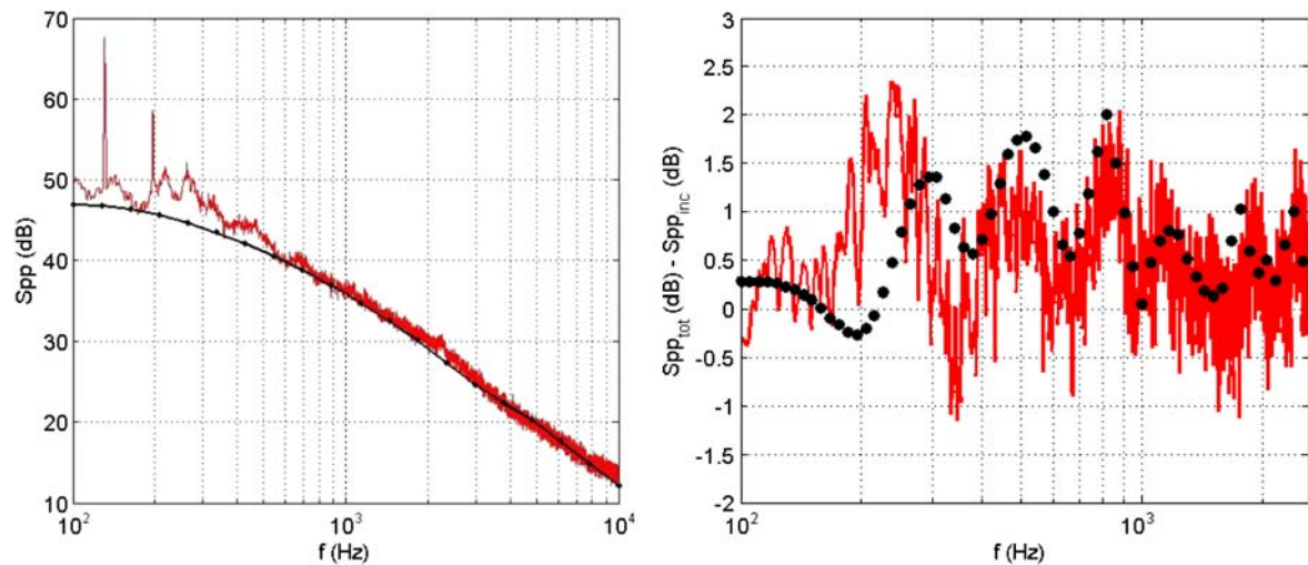
Fig. 10—Acoustic free-field spectra (left) at z = 3r measured (red) and semi-analytical model with 4 spanwise segments using inverse strip theory (black). Difference between total and free-field spectra (right). Measurements (line) and semi-analytical model combined with inverse strip theory and ATV approach (symbols).
