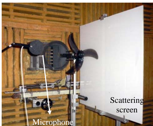
Fig. 8—Low-speed axial fan in the anechoic chamber (left). Acoustic PSD without (black) and with (red) turbulent flow at z = 3r . (right) 19 .
