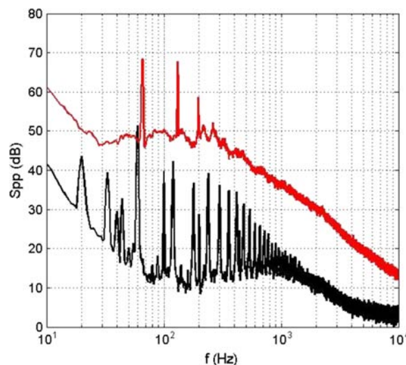
Fig. 8—Low-speed axial fan in the anechoic chamber (left). Acoustic PSD without (black) and with (red) turbulent flow at z = 3r . (right) 19 .
