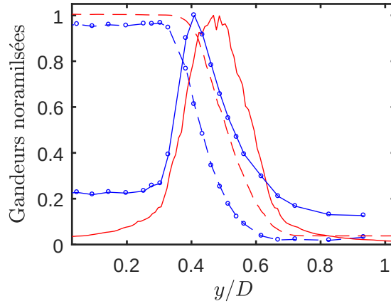
FIGURE 4.19 – Profils radiaux de : — — —, (\bar{\rho} - \rho_{amb})/(\rho_j - \rho_{amb}) ; — — —, \rho'_{rms}/\text{Max}(\rho'_{rms}) ; — — —, u/U_j ; — — —, u'_{rms}/\text{Max}(u'_{rms}) . z/D = 2 , M_j = 0.9 , T_0 = 29.7^\circ\text{C} , T_{amb} = 19.6^\circ\text{C} , tuyère C38.
