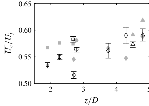
FIGURE 13. Spatially averaged convective velocity from the nozzle to the acoustic source normalised by the jet fully expanded velocity \overline{U}_c/U_j , against the acoustic source location z_N : \square , A1 mode; \circ , A2 mode; \diamond , b mode; \triangle , B mode; filled markers are from the wavenumber analysis; empty markers are from the phase analysis.
