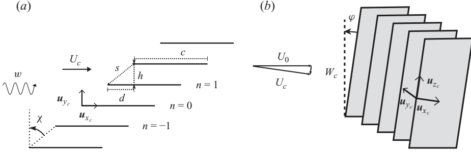
FIGURE 1. Geometry of the rectilinear-cascade model and incident velocity gust: (a) side view; (b) three-dimensional view. The spanwise velocity component W_c is non-zero only for swept blades. The blades are numbered from n = -\infty to n = +\infty .
