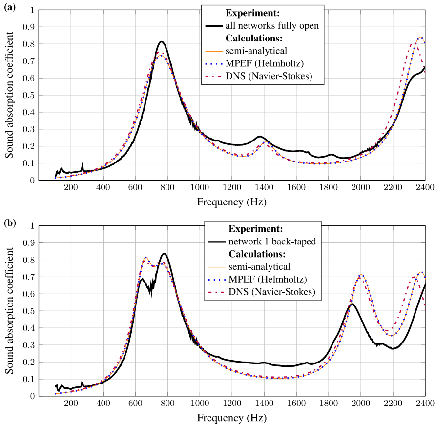
Fig. 14. Sound absorption by the 40 mm-thick sample of multi-tortuous metamaterial backed with a 10 mm air gap, for: (a) all networks fully open, or (b) network 1 taped at the back of the sample.
